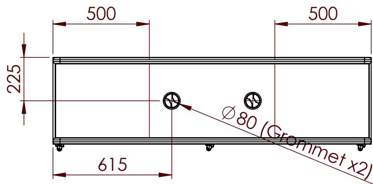
Bottom view Cable channel
